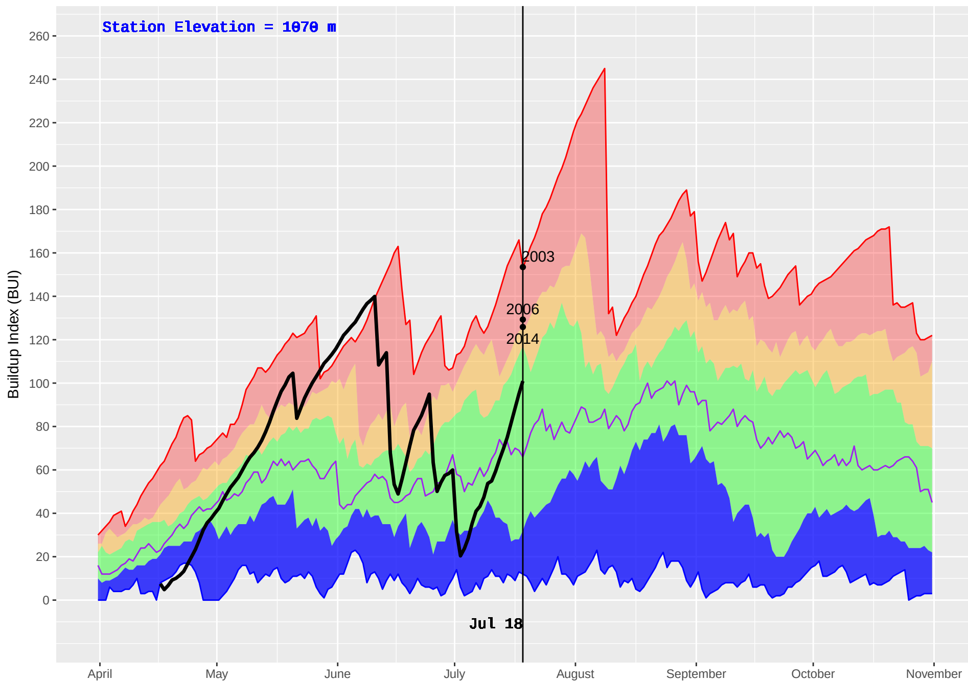
MEADOW LAKE (236) : Historical (1991–2016) and Current (2018) Daily Buildup Index (BUI)
