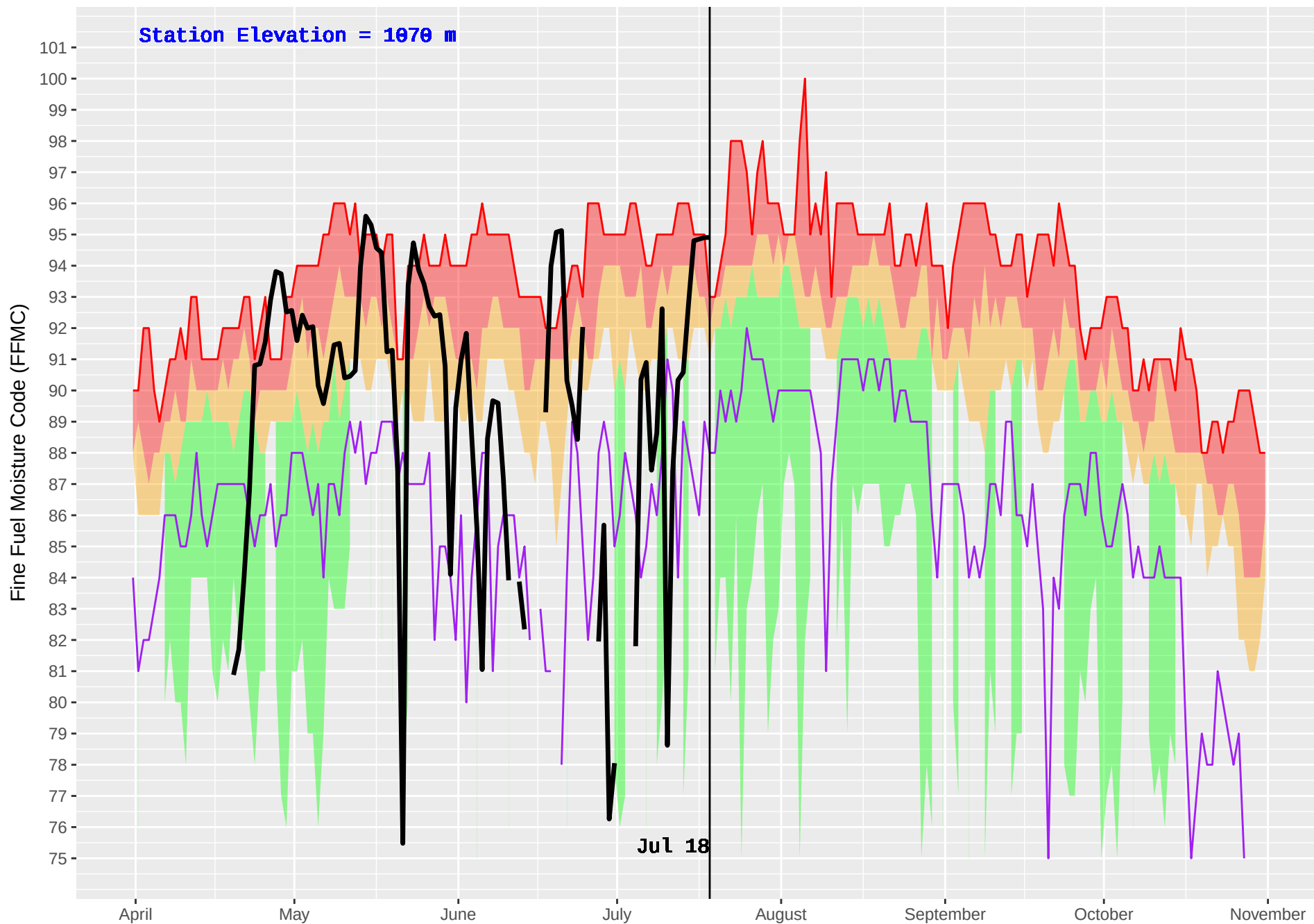
MEADOW LAKE (236) : Historical (1991–2016) and Current (2018) Daily Fine Fuel Moisture Code (FFMC)
