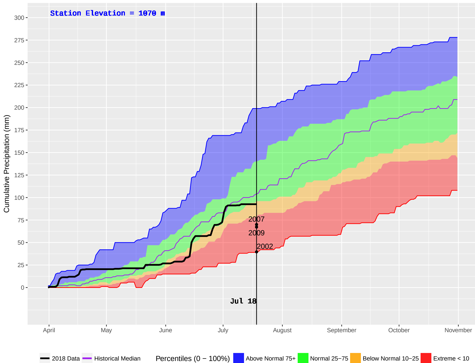
MEADOW LAKE (236) : Historical (1991–2016) and Current (2018) Daily Cumulative Precipitation
