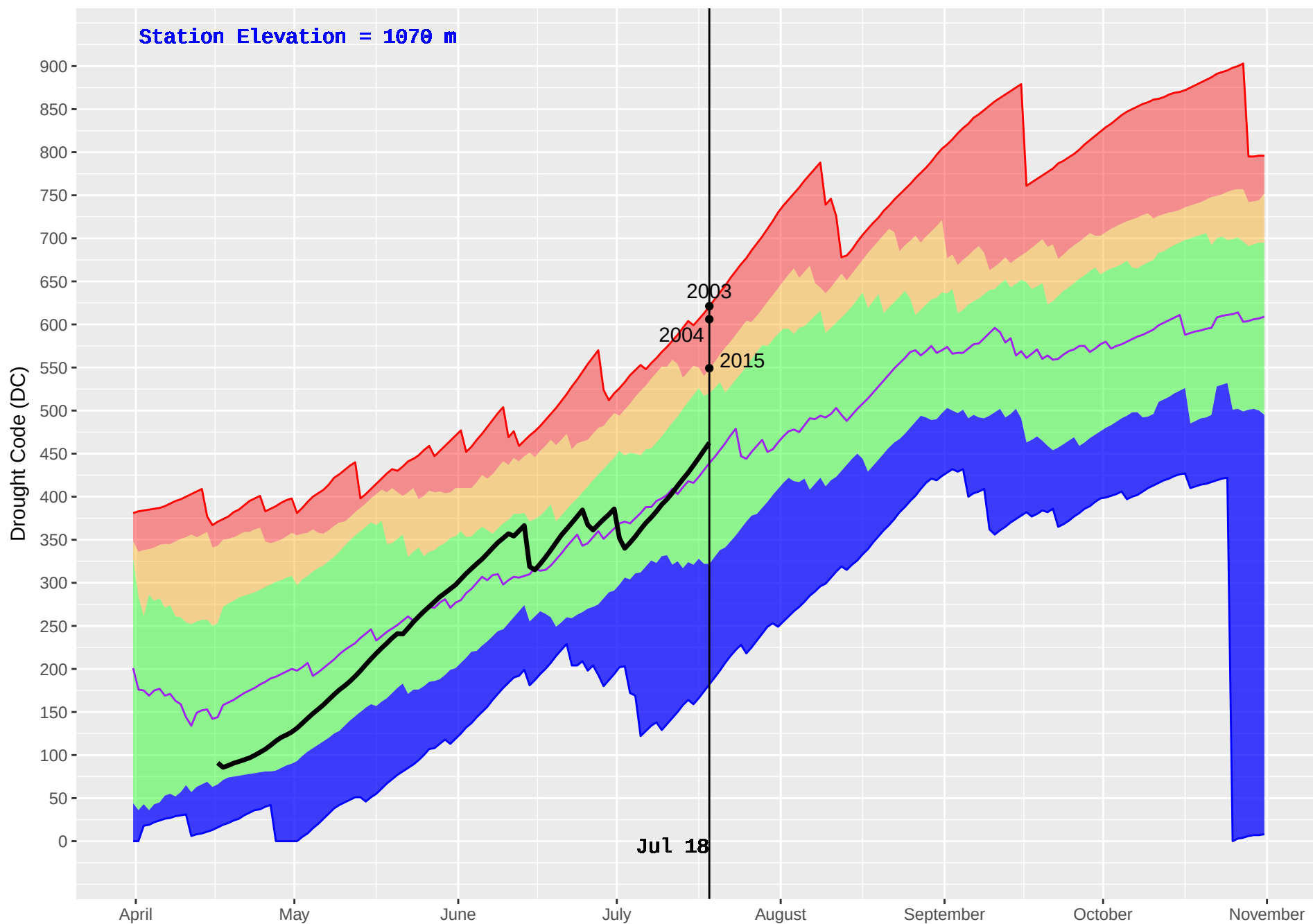
MEADOW LAKE (236) : Historical (1991–2016) and Current (2018) Daily Drought Code (DC)
